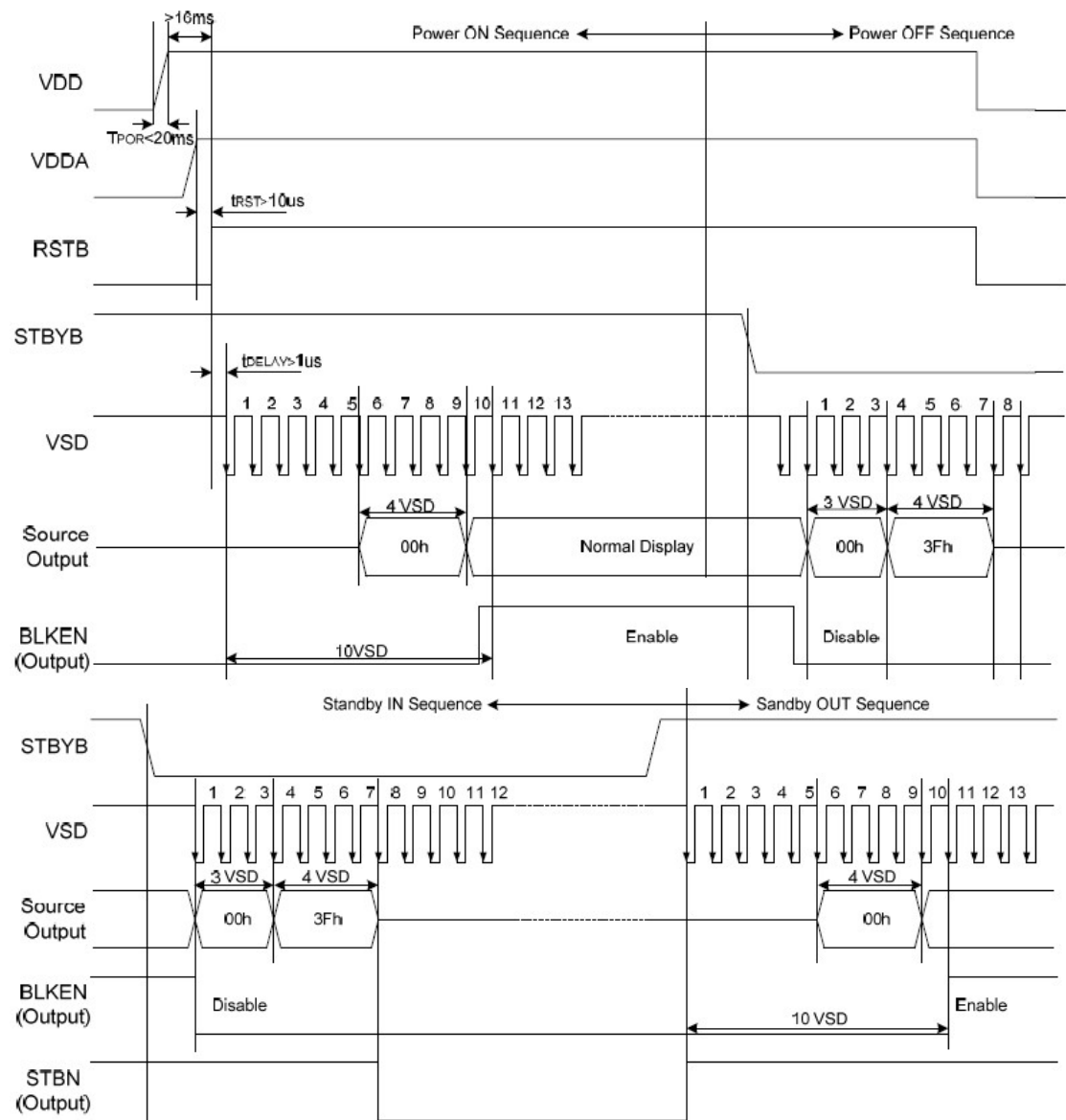
Power on sequence (VDD→VEE→VGH)
